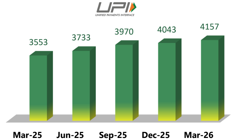
Count of UPI Transactions (Quarterly) (in lakhs)
